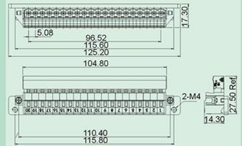
8EDGKRMA-5.08-20P-11-07AH
